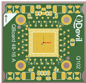
QDevil Q102 Daughter board 6.8x6.3 mm sample space
