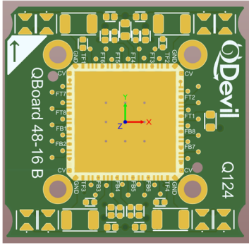
QDevil Q124 Daughter board 10.5x10.5 mm sample space
